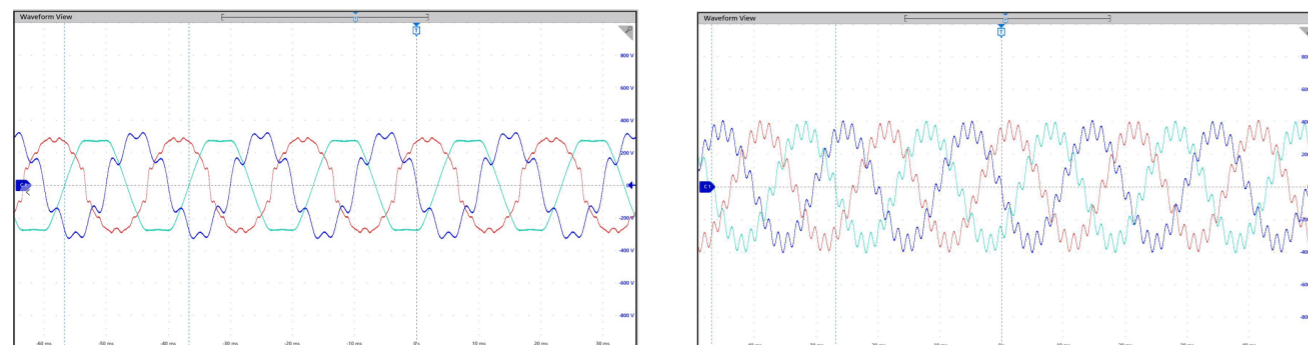
Harmonic Waveform
