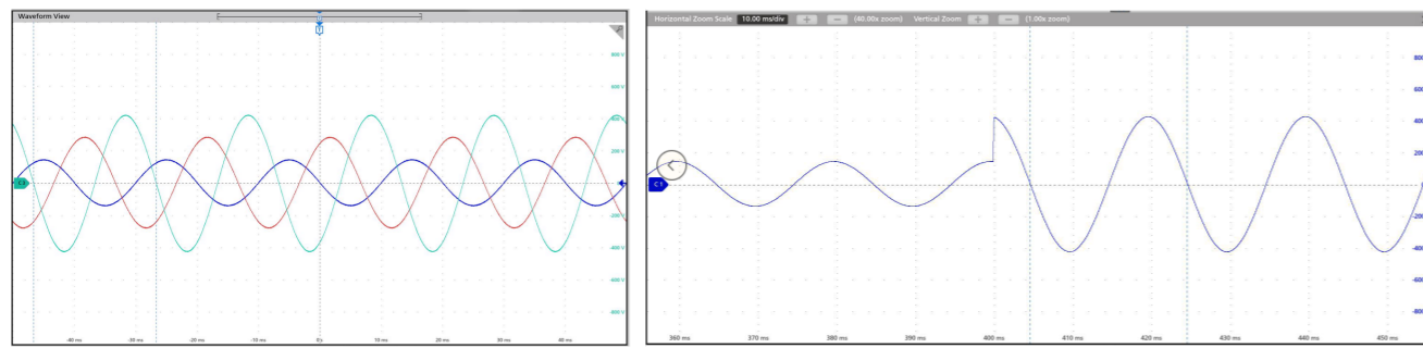
Three-phase Unbalance
