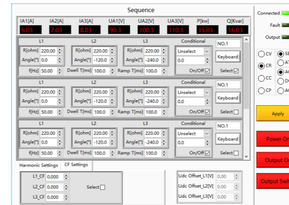
Sequence Programming
