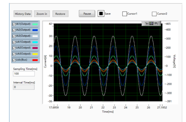
Waveform Display
