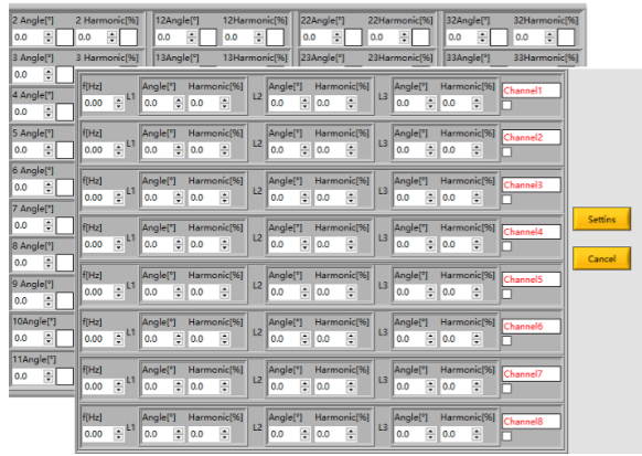
Harmonic/Inter-harmonic editing
