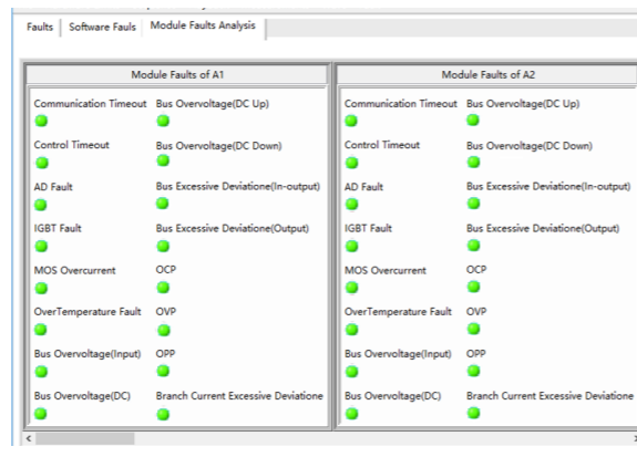
Fault Display
